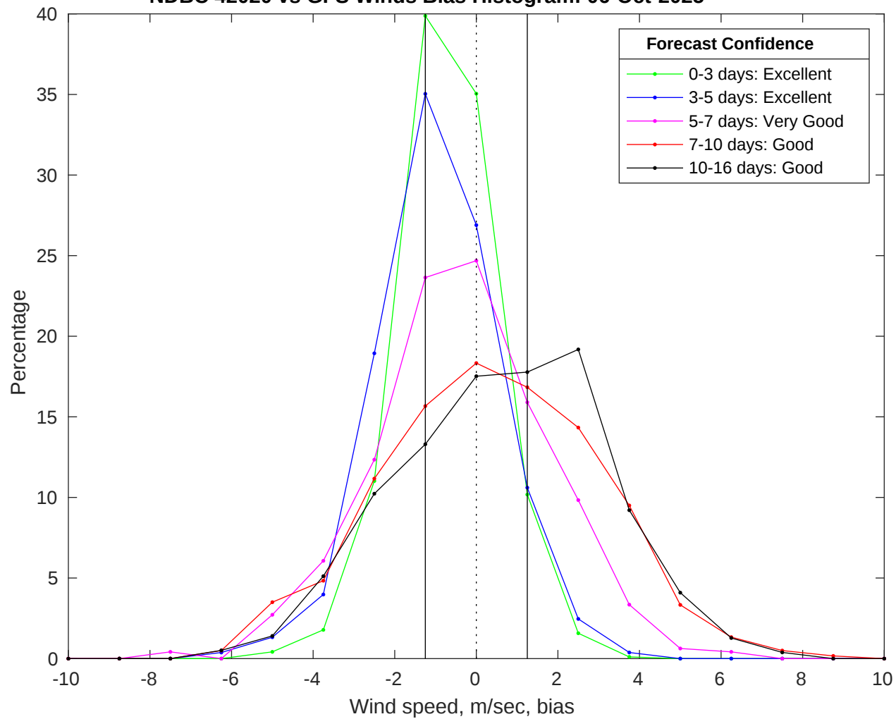
NDBC 42020 vs GFS Winds Bias Histogram: 06-Oct-2025
