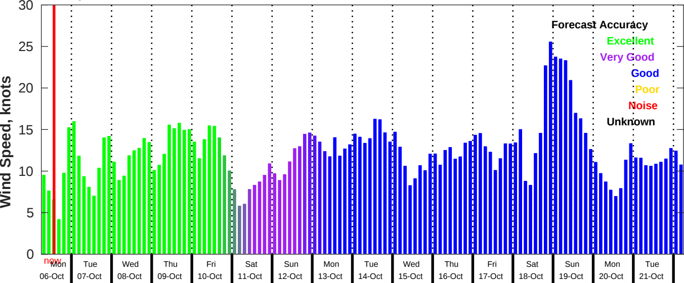
GFS Wind Speed Forecast for NDBC 42020 from 06-Oct-2025 06:00:00 to 22-Oct-2025 06:00:00
