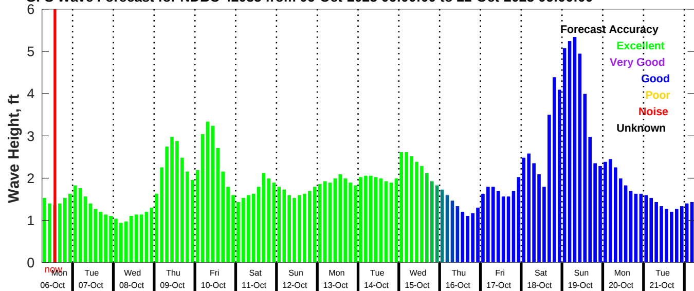
GFS Wave Forecast for NDBC 42035 from 06-Oct-2025 06:00:00 to 22-Oct-2025 06:00:00
