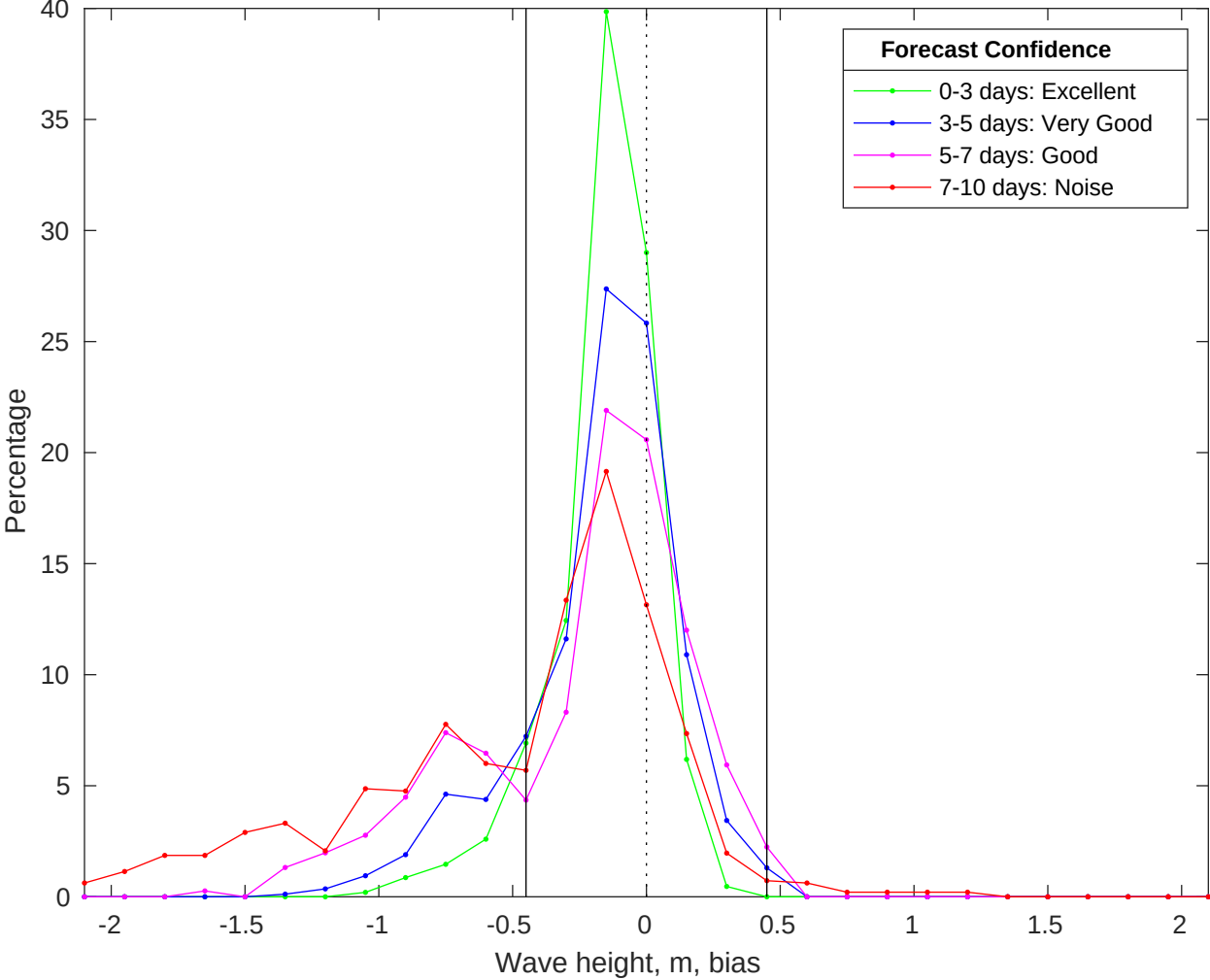
NDBC 42036 vs CMEMS Waves Bias Histogram: 06-Oct-2025
