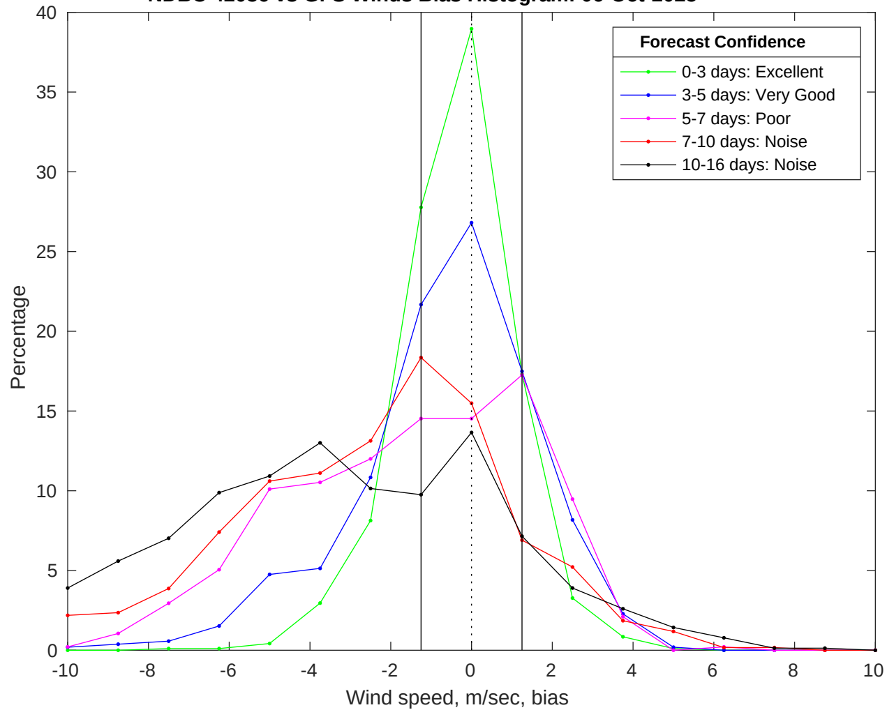
NDBC 42036 vs GFS Winds Bias Histogram: 06-Oct-2025
