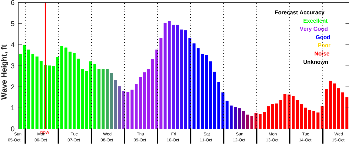
CMEMS Wave Forecast for NDBC 42036 from 05-Oct-2025 19:00:00 to 15-Oct-2025 19:00:00
