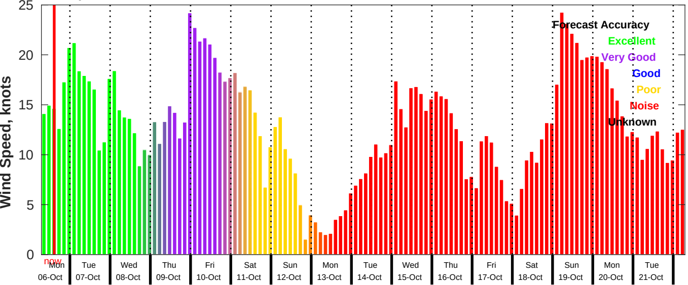
GFS Wind Speed Forecast for NDBC 42036 from 06-Oct-2025 07:00:00 to 22-Oct-2025 07:00:00
