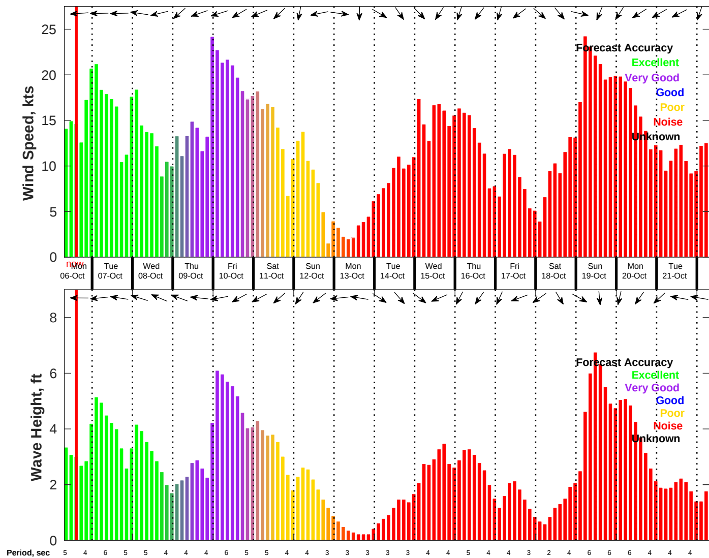
Wind & Wave Forecast for NDBC 42036 from 06-Oct-2025 07:00:00 to 22-Oct-2025 07:00:00
