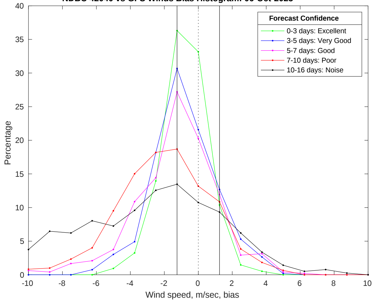
NDBC 42040 vs GFS Winds Bias Histogram: 06-Oct-2025
