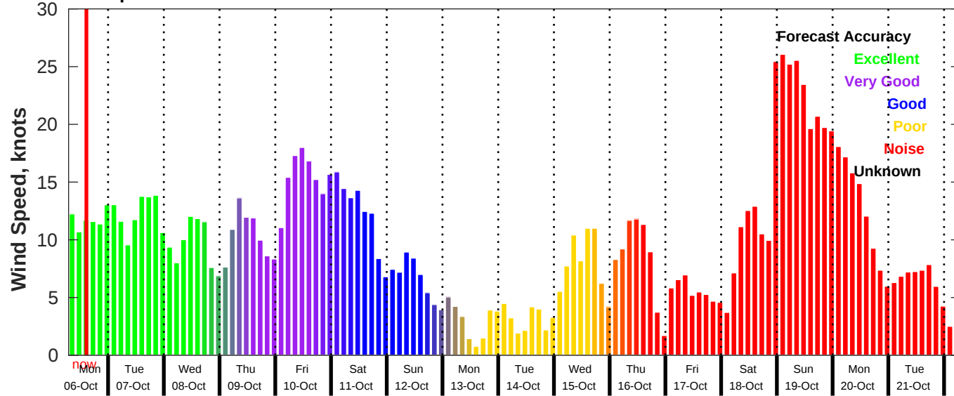
GFS Wind Speed Forecast for NDBC 42040 from 06-Oct-2025 07:00:00 to 22-Oct-2025 07:00:00
