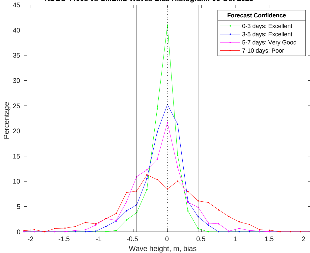
NDBC 44008 vs CMEMS Waves Bias Histogram: 06-Oct-2025
