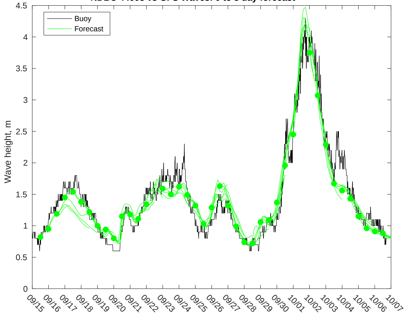
NDBC 44008 vs GFS Waves: 0 to 3 day forecast
