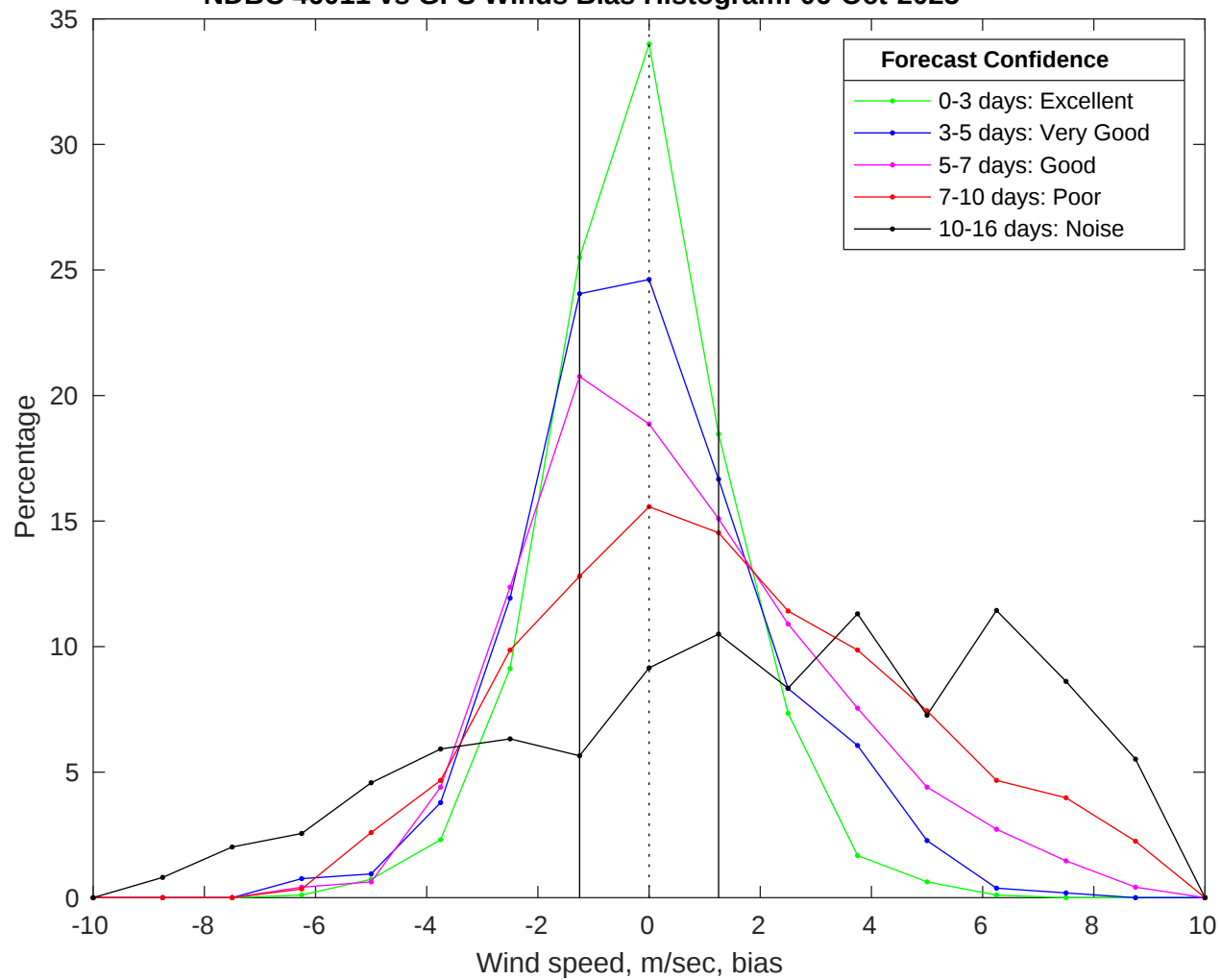
NDBC 46011 vs GFS Winds Bias Histogram: 06-Oct-2025
