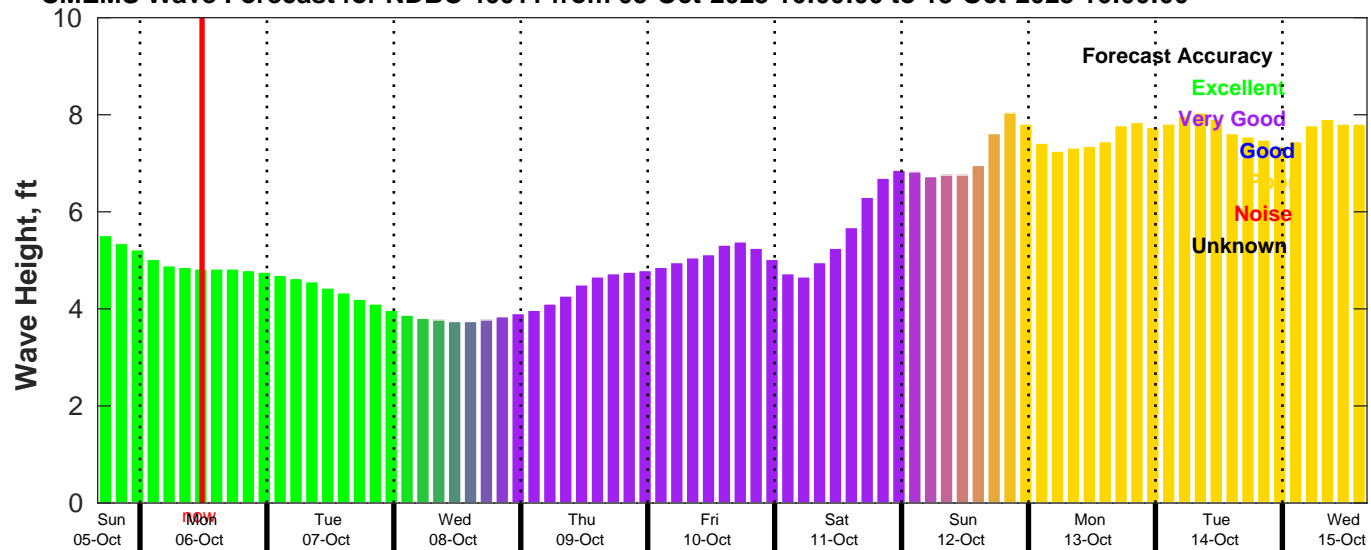
CMEMS Wave Forecast for NDBC 46011 from 05-Oct-2025 16:00:00 to 15-Oct-2025 16:00:00
