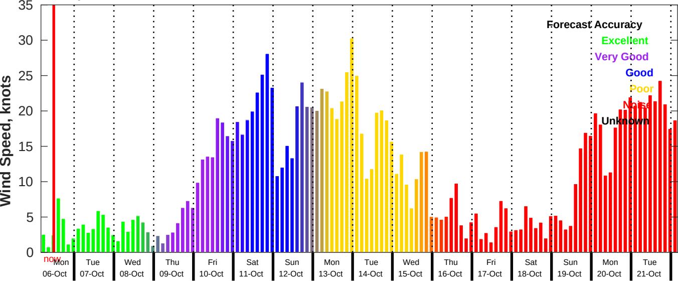
GFS Wind Speed Forecast for NDBC 46011 from 06-Oct-2025 04:00:00 to 22-Oct-2025 04:00:00
