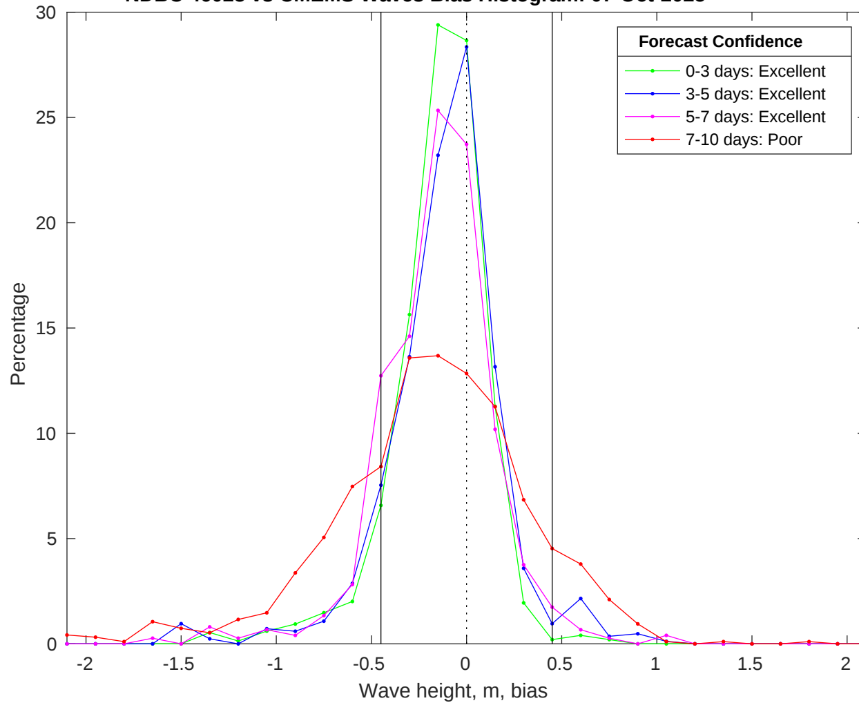
NDBC 46028 vs CMEMS Waves Bias Histogram: 07-Oct-2025
