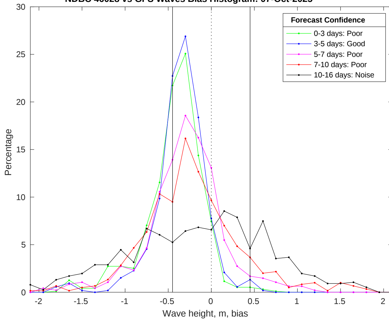
NDBC 46028 vs GFS Waves Bias Histogram: 07-Oct-2025
