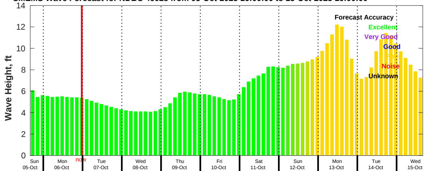
CMEMS Wave Forecast for NDBC 46028 from 05-Oct-2025 16:00:00 to 15-Oct-2025 16:00:00
