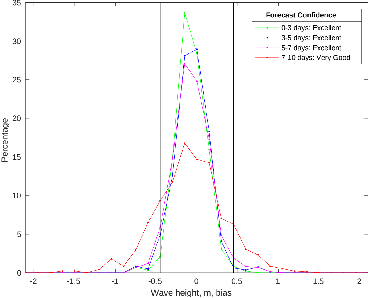
NDBC 46054 vs CMEMS Waves Bias Histogram: 07-Oct-2025
