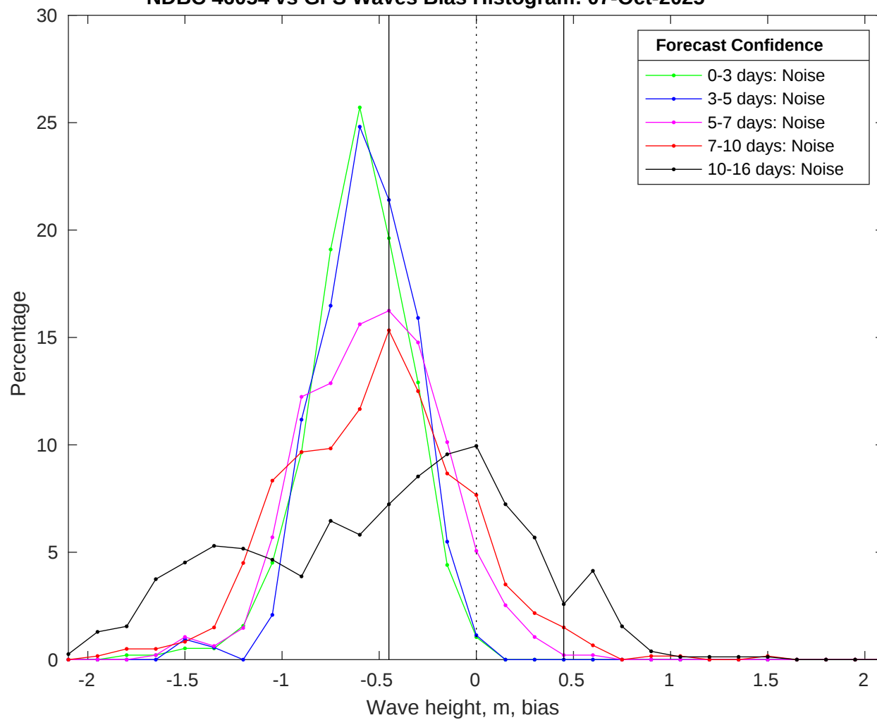
NDBC 46054 vs GFS Waves Bias Histogram: 07-Oct-2025
