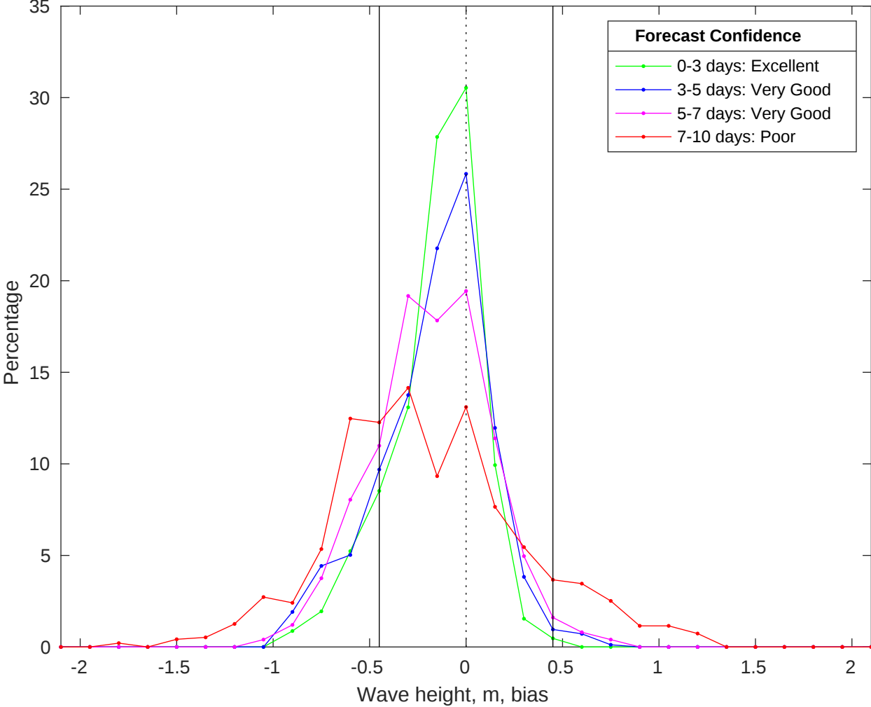
NDBC 46069 vs CMEMS Waves Bias Histogram: 07-Oct-2025
