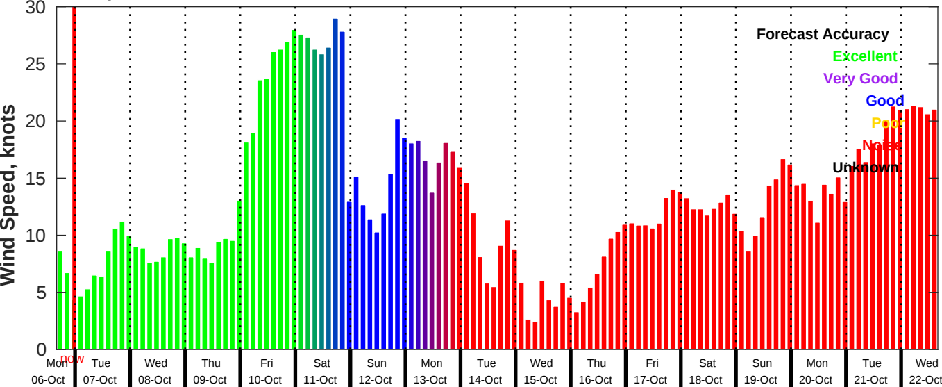
GFS Wind Speed Forecast for NDBC 46069 from 06-Oct-2025 16:00:00 to 22-Oct-2025 16:00:00
