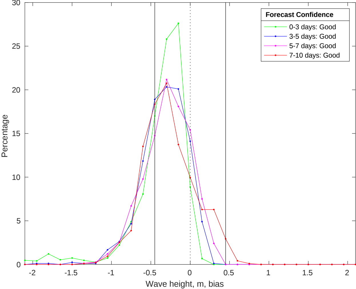
NDBC 51209 vs CMEMS Waves Bias Histogram: 07-Oct-2025
