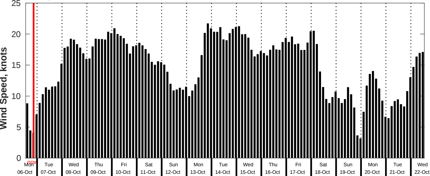
GFS Wind Speed Forecast for NDBC 51209 from 06-Oct-2025 13:00:00 to 22-Oct-2025 13:00:00
