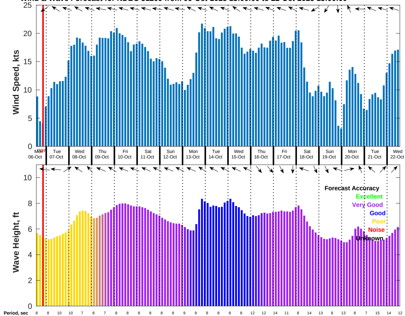
Wind & Wave Forecast for NDBC 51209 from 06-Oct-2025 13:00:00 to 22-Oct-2025 13:00:00
