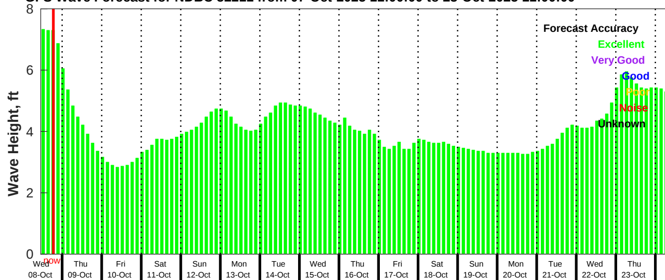
GFS Wave Forecast for NDBC 52211 from 07-Oct-2025 11:00:00 to 23-Oct-2025 11:00:00
