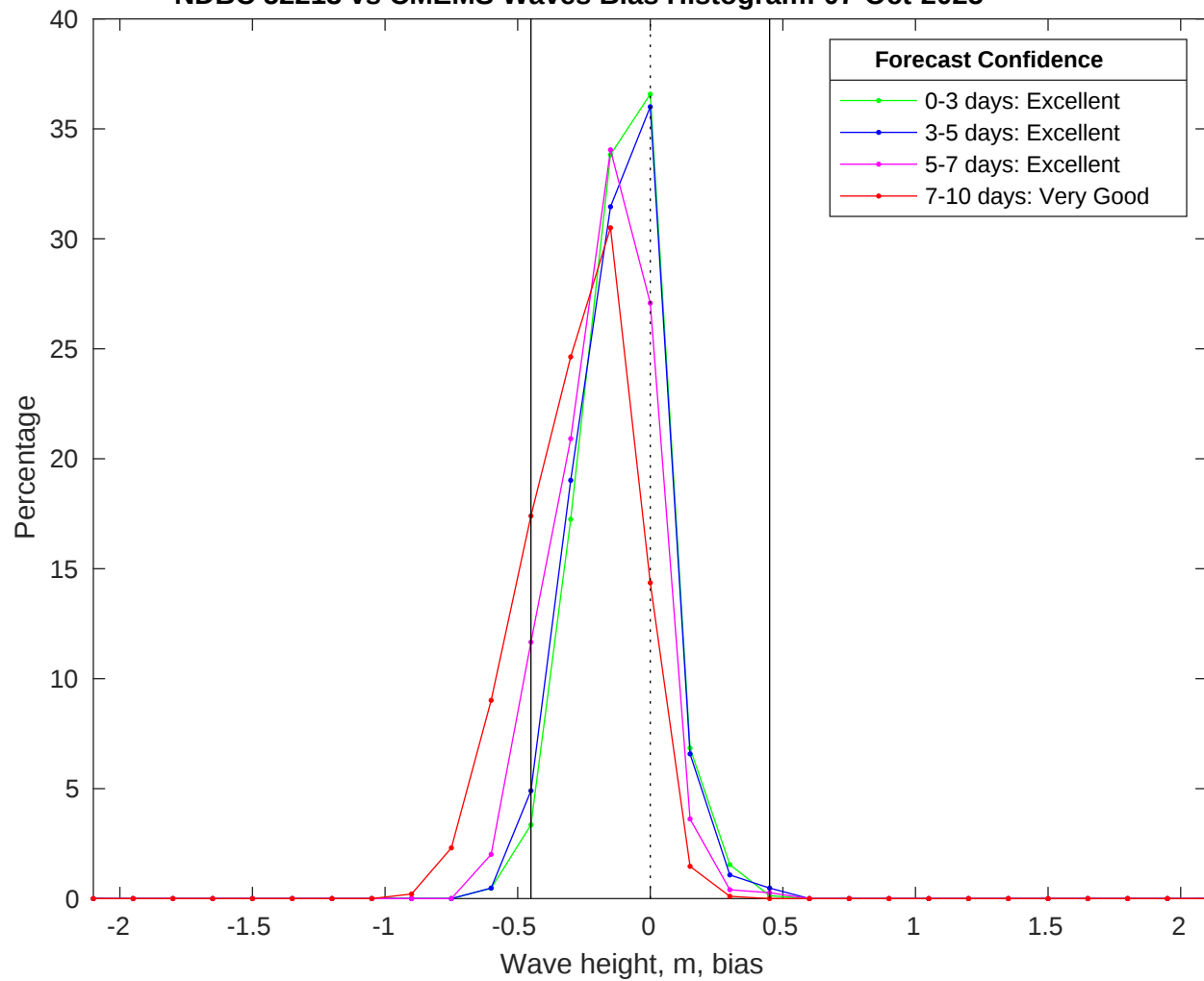
NDBC 52213 vs CMEMS Waves Bias Histogram: 07-Oct-2025
