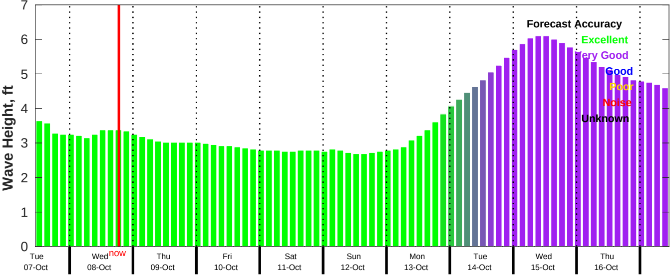
CMEMS Wave Forecast for NDBC 52213 from 06-Oct-2025 11:00:00 to 16-Oct-2025 11:00:00
