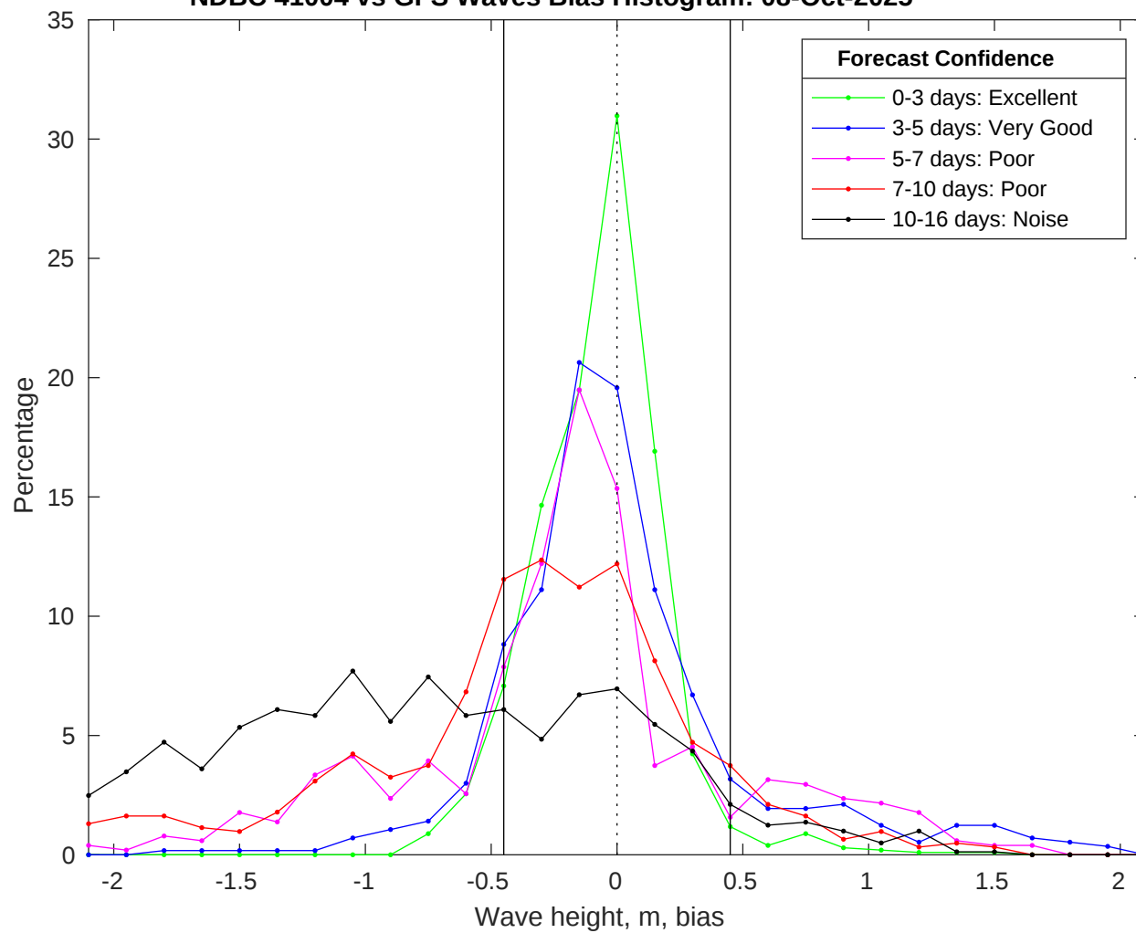
NDBC 41004 vs GFS Waves Bias Histogram: 08-Oct-2025
