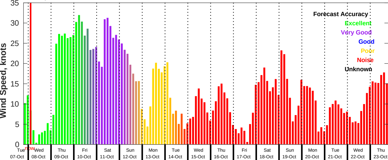
GFS Wind Speed Forecast for NDBC 41004 from 07-Oct-2025 19:00:00 to 23-Oct-2025 19:00:00
