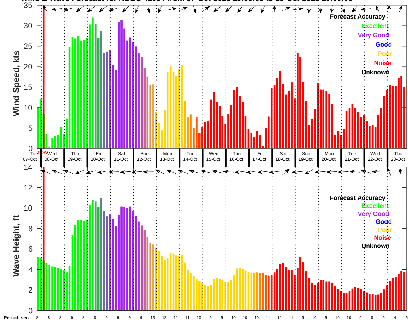
Wind & Wave Forecast for NDBC 41004 from 07-Oct-2025 19:00:00 to 23-Oct-2025 19:00:00
