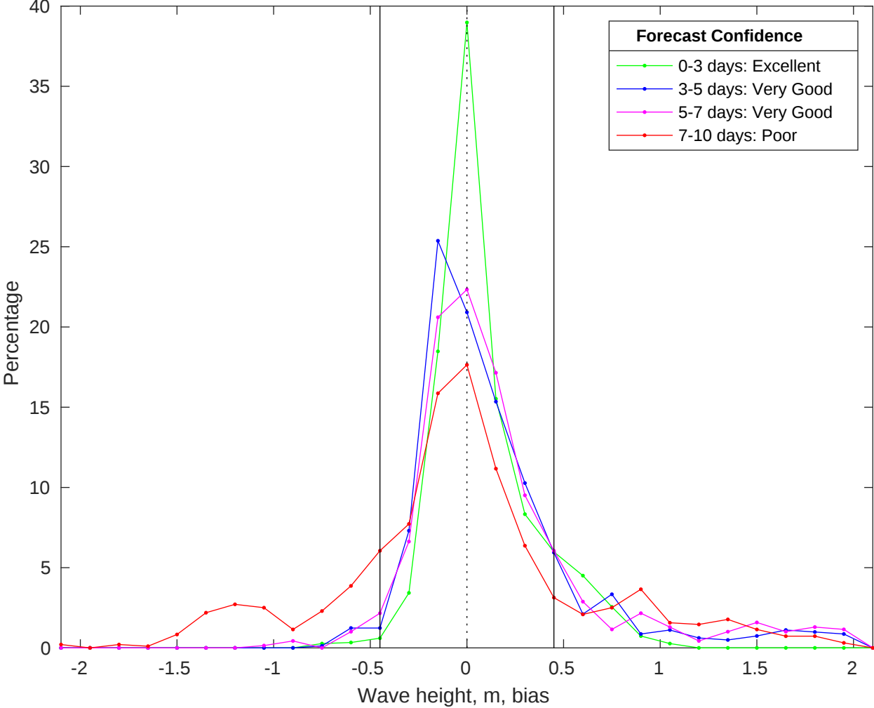
NDBC 41013 vs CMEMS Waves Bias Histogram: 07-Oct-2025
