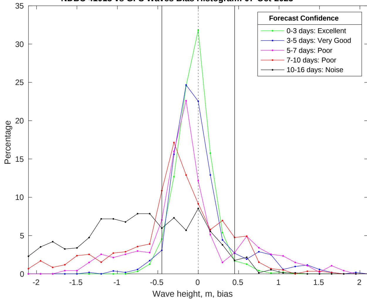
NDBC 41013 vs GFS Waves Bias Histogram: 07-Oct-2025
