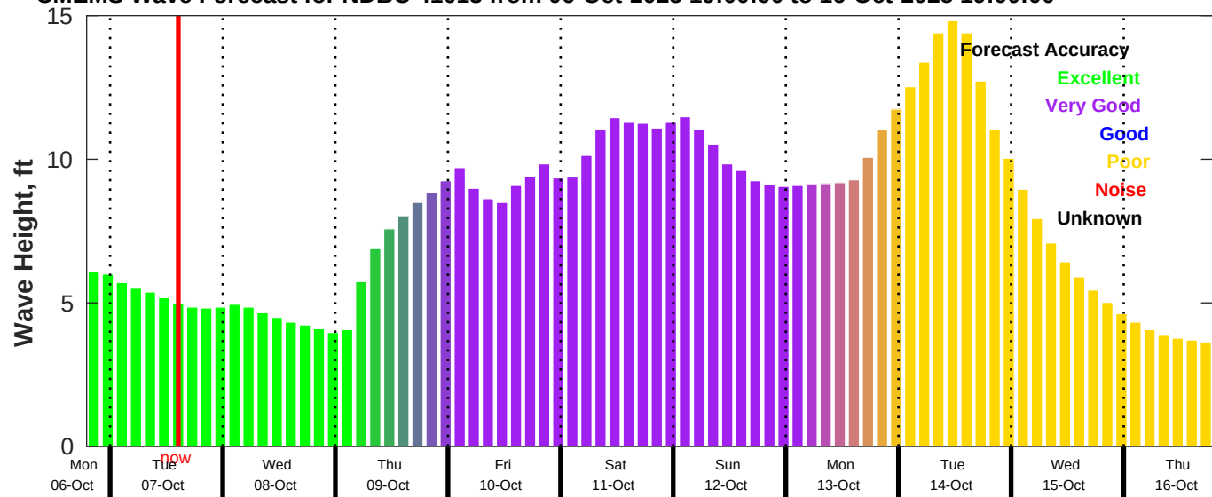
CMEMS Wave Forecast for NDBC 41013 from 06-Oct-2025 19:00:00 to 16-Oct-2025 19:00:00
