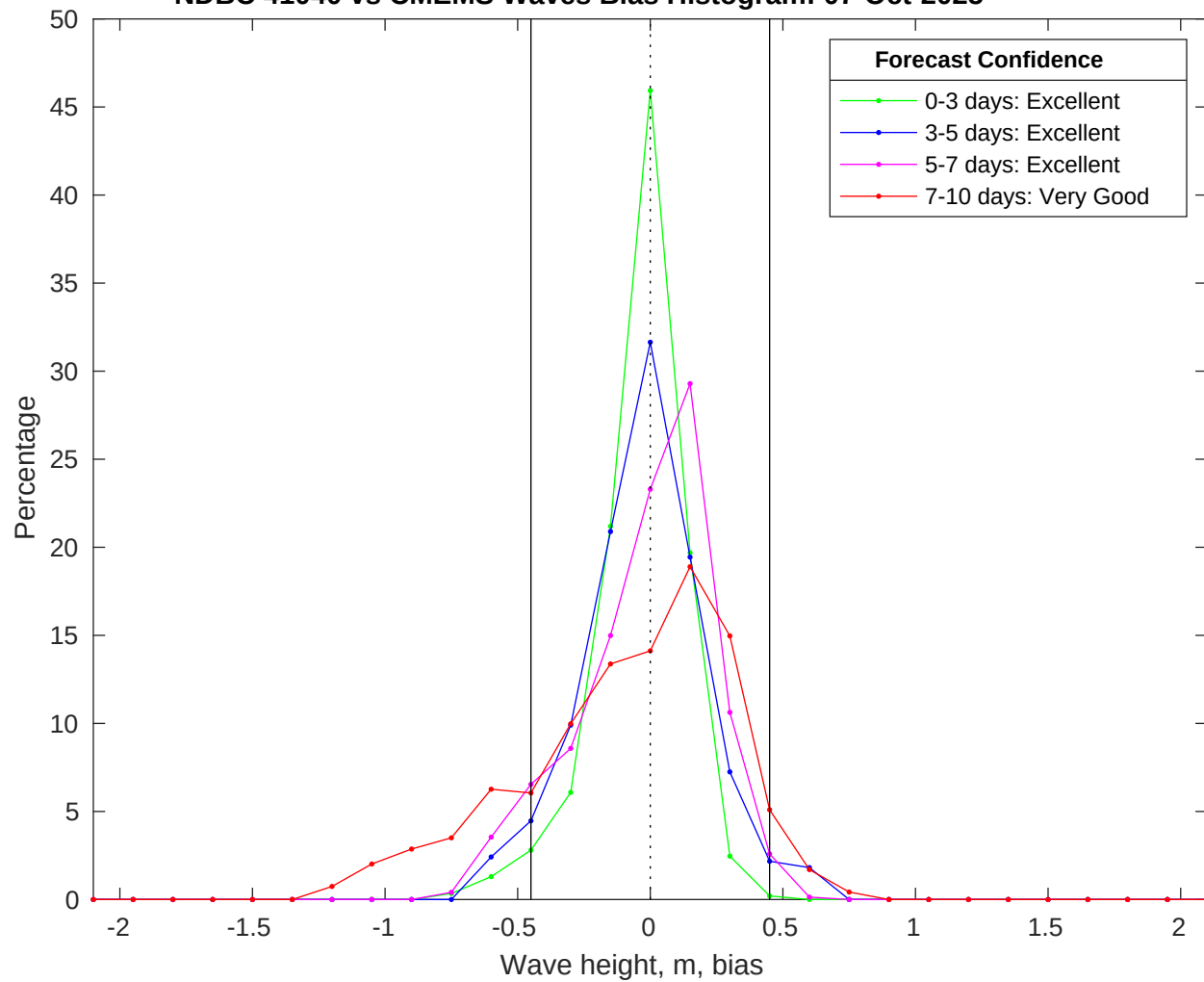
NDBC 41040 vs CMEMS Waves Bias Histogram: 07-Oct-2025
