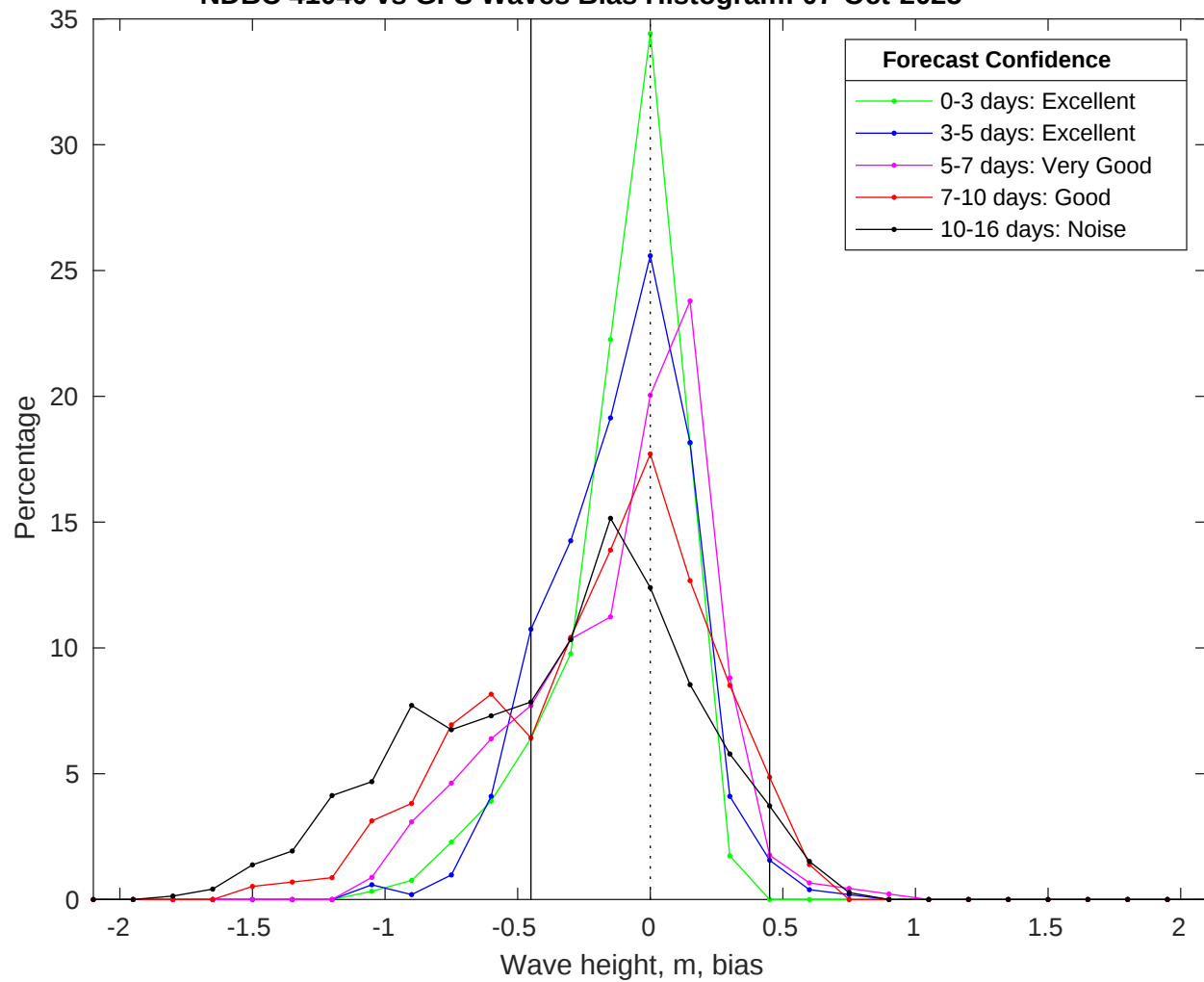
NDBC 41040 vs GFS Waves Bias Histogram: 07-Oct-2025
