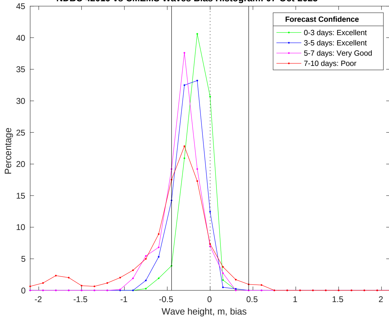
NDBC 42019 vs CMEMS Waves Bias Histogram: 07-Oct-2025
