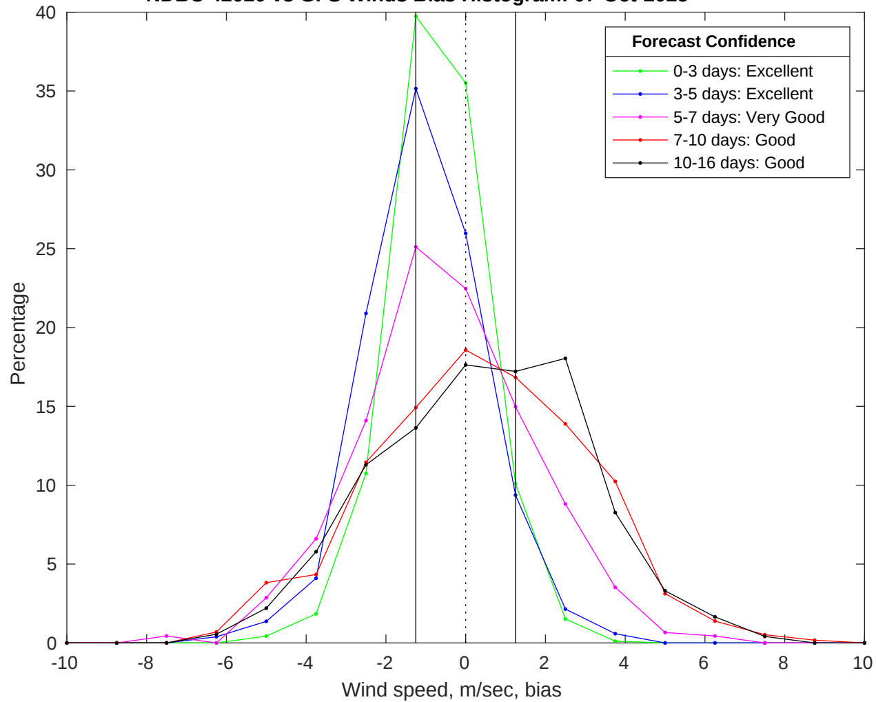
NDBC 42020 vs GFS Winds Bias Histogram: 07-Oct-2025
