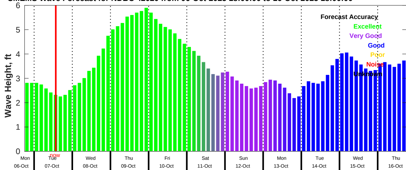
CMEMS Wave Forecast for NDBC 42020 from 06-Oct-2025 18:00:00 to 16-Oct-2025 18:00:00
