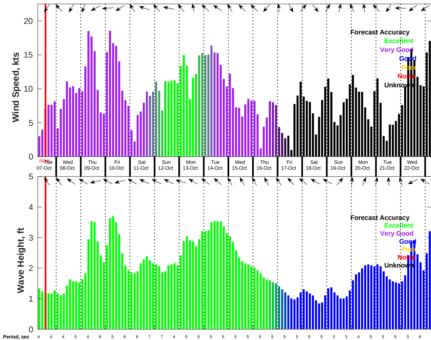
Wind & Wave Forecast for NDBC 42035 from 07-Oct-2025 06:00:00 to 23-Oct-2025 06:00:00
