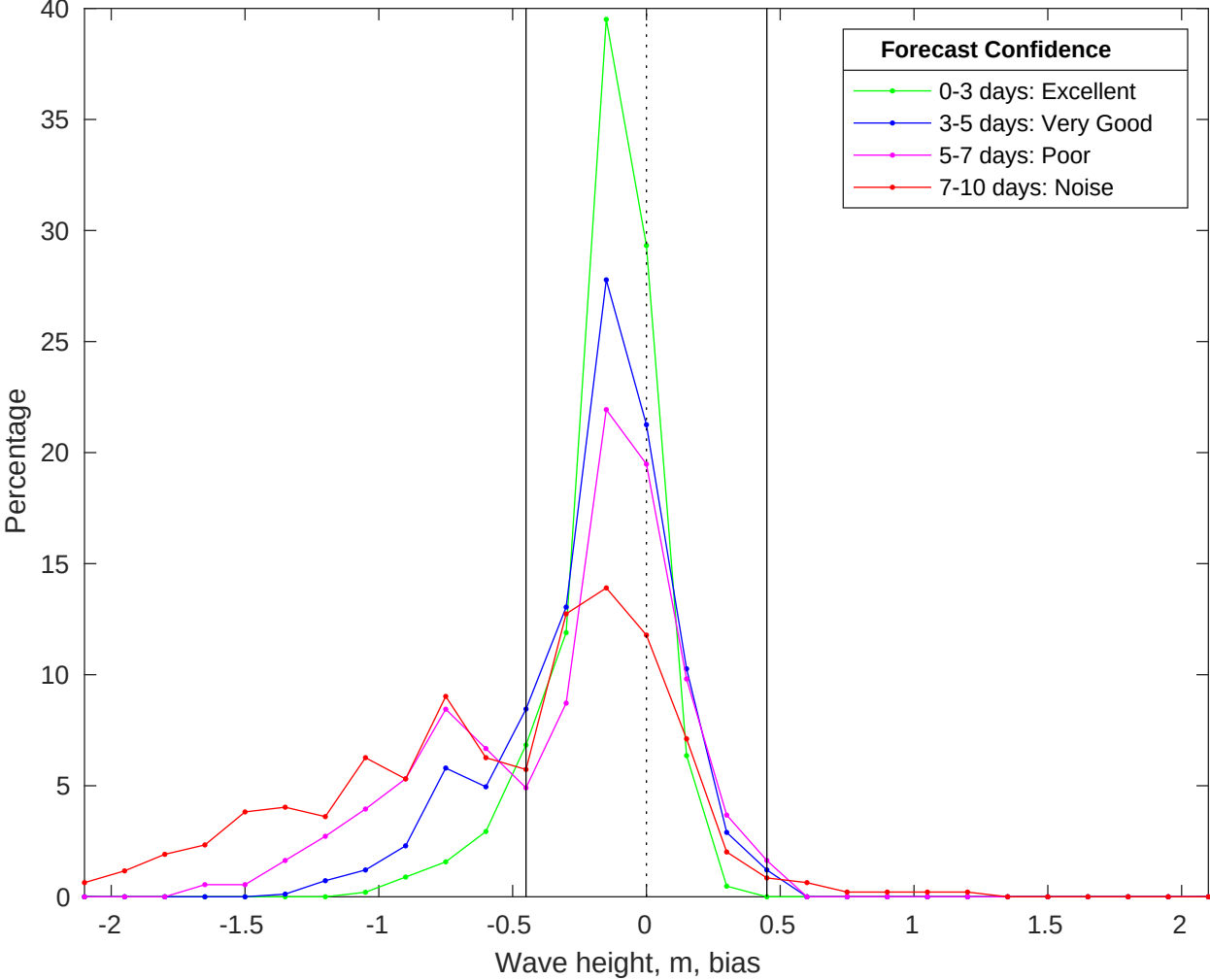
NDBC 42036 vs CMEMS Waves Bias Histogram: 07-Oct-2025
