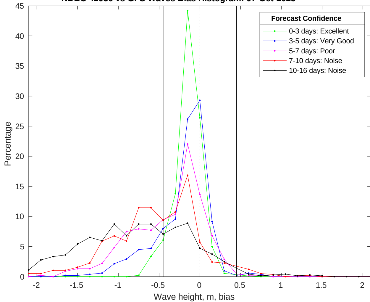
NDBC 42036 vs GFS Waves Bias Histogram: 07-Oct-2025
