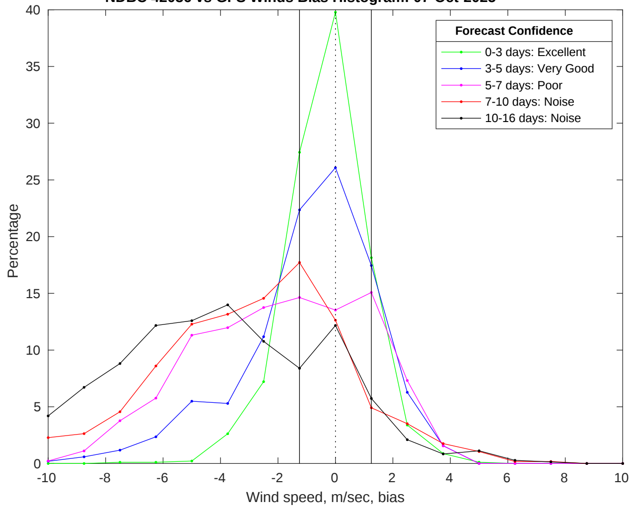
NDBC 42036 vs GFS Winds Bias Histogram: 07-Oct-2025
