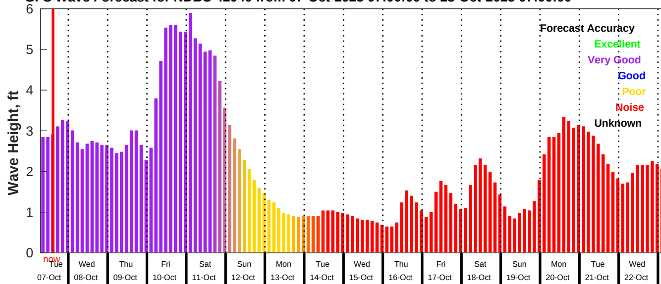
GFS Wave Forecast for NDBC 42040 from 07-Oct-2025 07:00:00 to 23-Oct-2025 07:00:00
