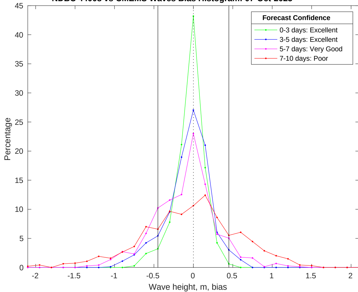
NDBC 44008 vs CMEMS Waves Bias Histogram: 07-Oct-2025
