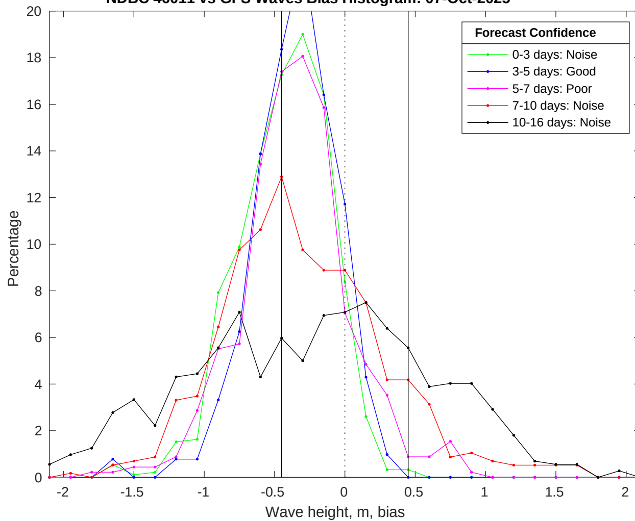
NDBC 46011 vs GFS Waves Bias Histogram: 07-Oct-2025
