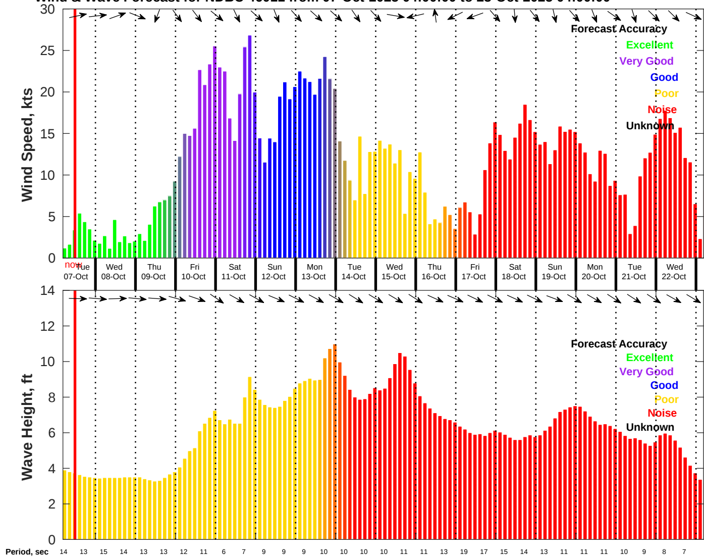
Wind & Wave Forecast for NDBC 46011 from 07-Oct-2025 04:00:00 to 23-Oct-2025 04:00:00
