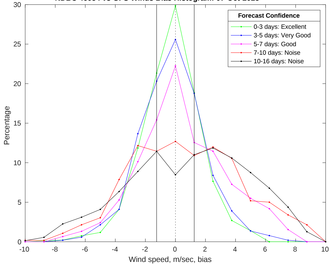
NDBC 46054 vs GFS Winds Bias Histogram: 07-Oct-2025
