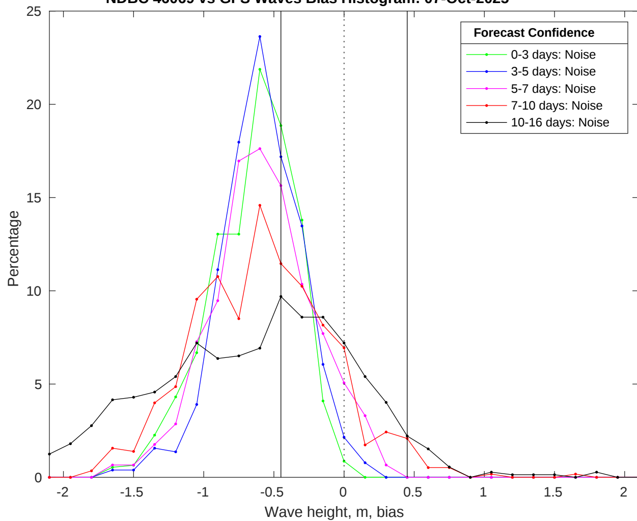
NDBC 46069 vs GFS Waves Bias Histogram: 07-Oct-2025
