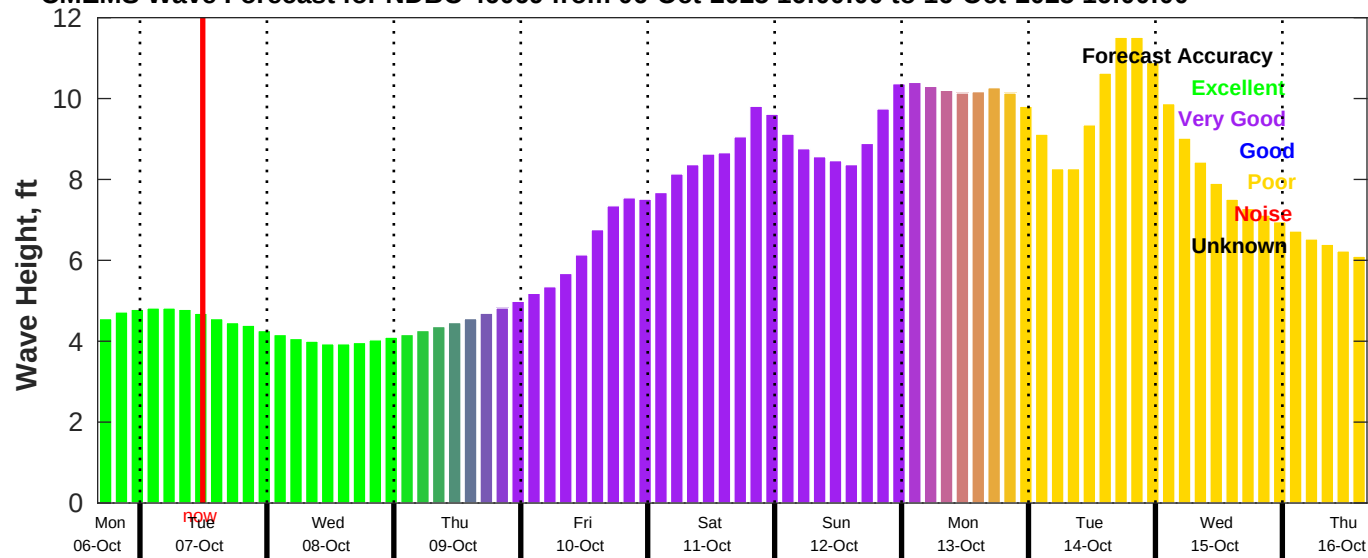
CMEMS Wave Forecast for NDBC 46069 from 06-Oct-2025 16:00:00 to 16-Oct-2025 16:00:00
